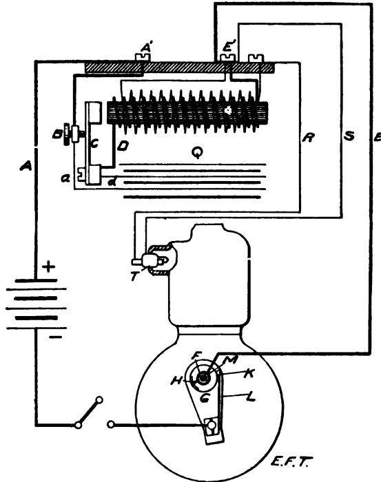
FIG. 336.—The Benz Jump-Spark Circuit. Unlike the De Dion system just described, both the primary and secondary circuits are carried by visible leads, no part of either being grounded to the frame. The circuit emerging from the positive pole of the battery passes through wire, A, to binding post, A' on the coil, to one contact at B of the trembler, C, thence through C and D to the primary winding of the coil; then through a and d through the condenser, Q. The other terminal of the primary winding emerges from binding post, E', passing over lead wire, E, to sleeve, M, of the rotary cam, G. The sleeve, M, is in electrical contact with the metallic section, H, on the circumference of the cam, being turned on the spindle, F, so as to periodically make contact with the head, K, of the trembler spring, L. The secondary circuit is completed through lead wires, R and S, to the two terminals of the plug, T.
